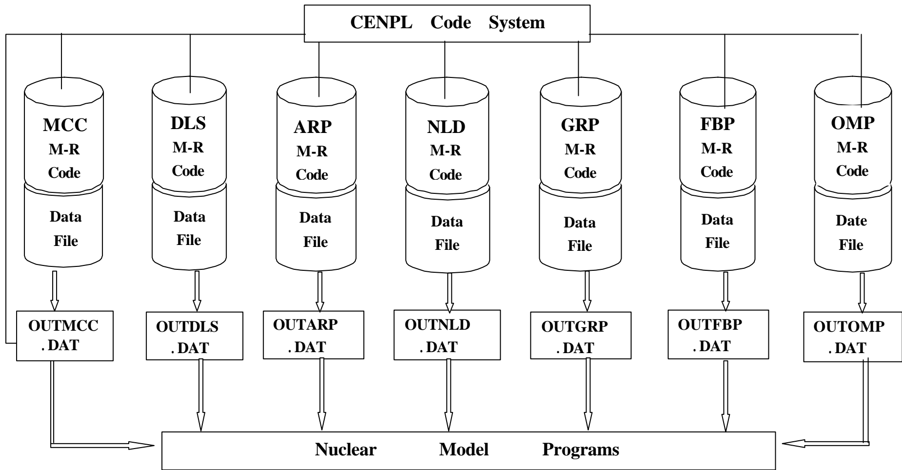
Figure1 : Chinese Evaluated Nuclear Parameter Library
