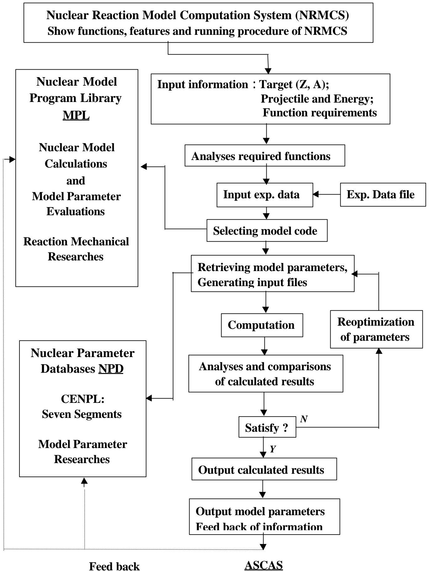
Figure2 : Nuclear Reaction Model Computation System
